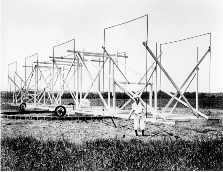
Fig. 1.2 Karl Jansky and his rotating Bruce Array known as the “merry-go-round,” which he used in 1932 to detect radio emission from the Milky Way Galaxy. Credit: NRAO/AUI/NSF
