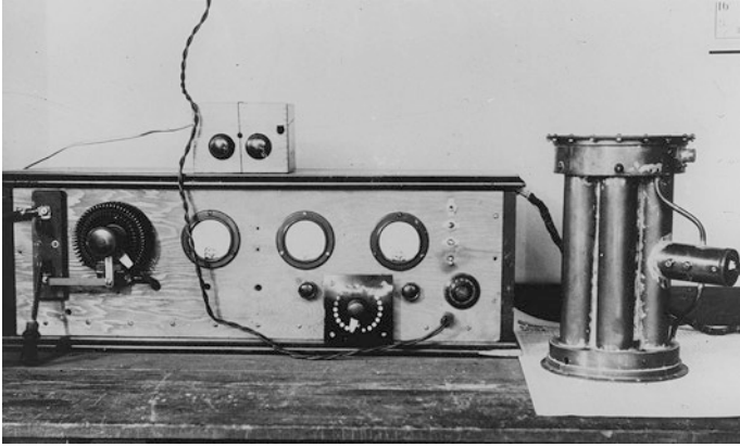
Fig. 1.6 Some of Reber's Wheaton equipment used to study cosmic radio emission. On the left is his receiver monitor and control system. On the right is his 160 MHz amplifier. Credit: NRAO/AUI/NSF
