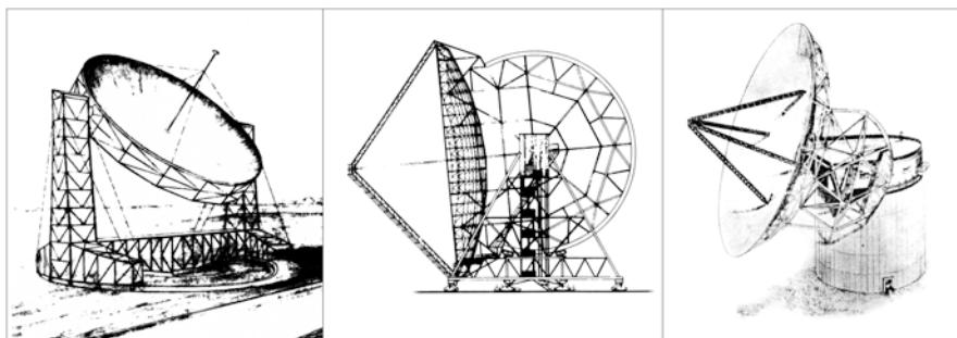
Fig. 4.6 Left to right: Feld, Husband, and Kennedy telescope designs for the Green Bank antenna. Credit: NRAO/AUI/NSF
