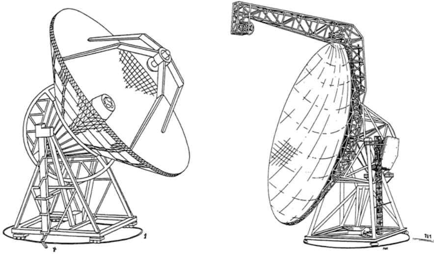
Fig. 9.12 100 meter telescope concepts. Right: axially symmetrical design; Left: offset reflector 100 design. Credit: NRAO/AUI/NSF
