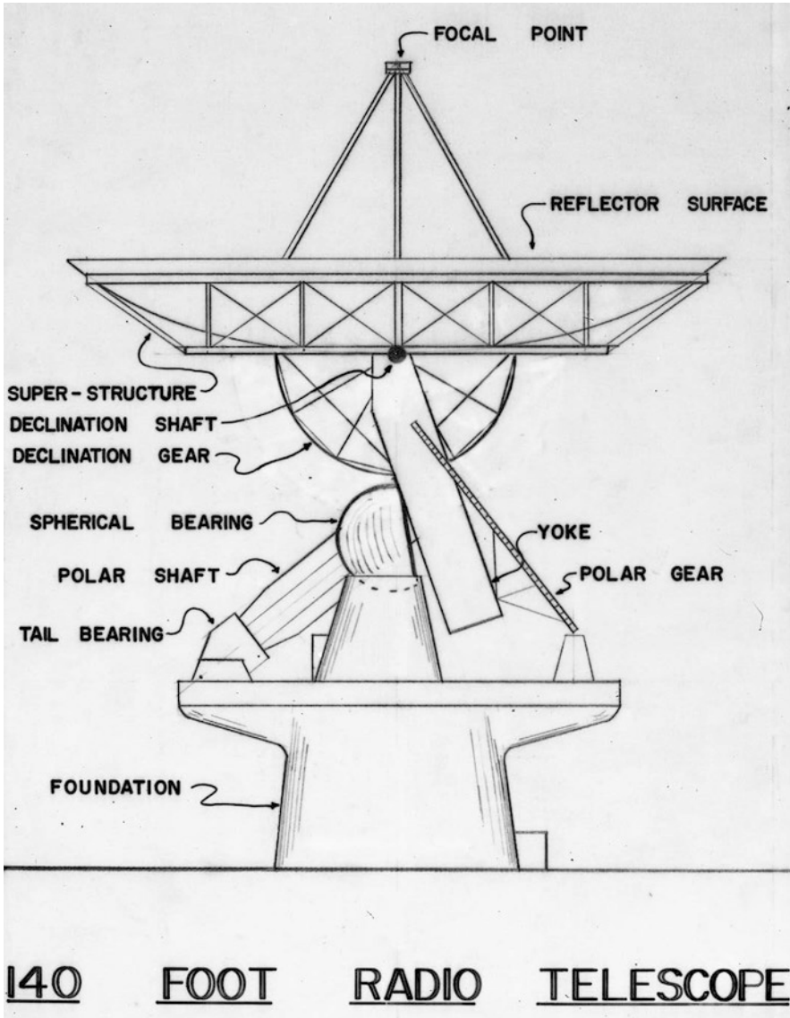
Fig. 4.7 Ned Ashton design for the 140 Foot Telescope. Credit: NRAO/AUI/NSF
