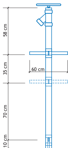
Figure 4.6 Schematic of the Sludge Gulper (Tilley et al. , 2014).
