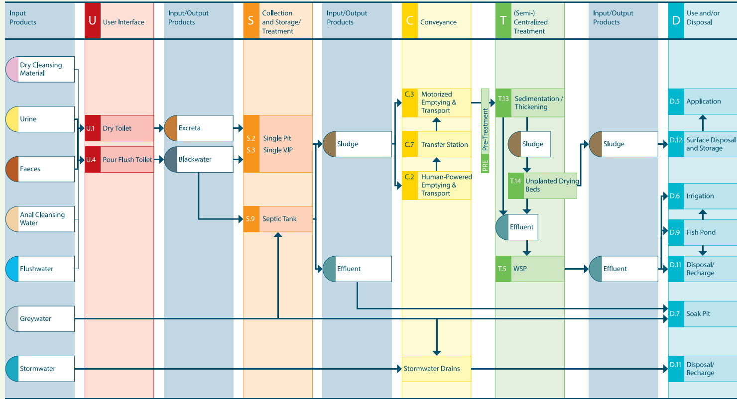
Figure 17.11 Example diagram of a faecal sludge sanitation system proposal (adapted from Tilley et al. , 2014).
