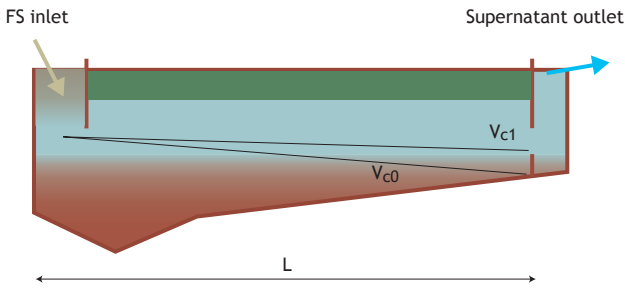
Figure 6.3 Schematic of the final settling velocity ( V_c ) needed for a particle to settle in a tank of length L .
