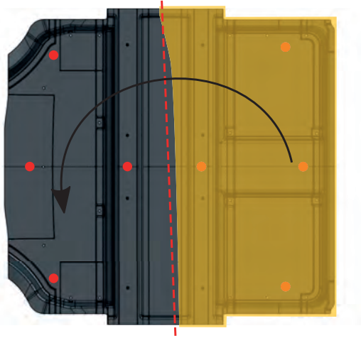
Figure 7.35: Schematic of the asymmetric bending of the component during demolding
