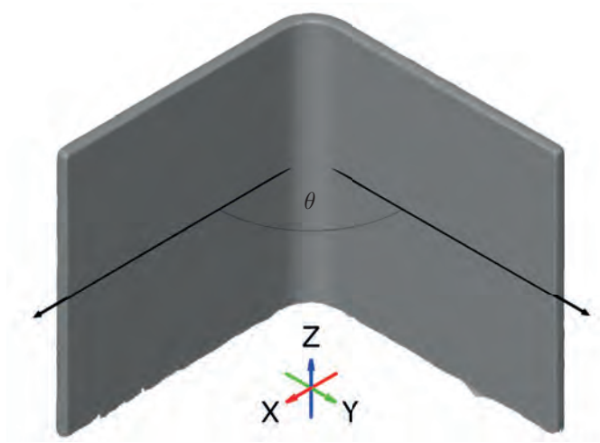
Figure 7.10: Evaluation of the spring-in angle of RTM specimens using GOM Inspect software
