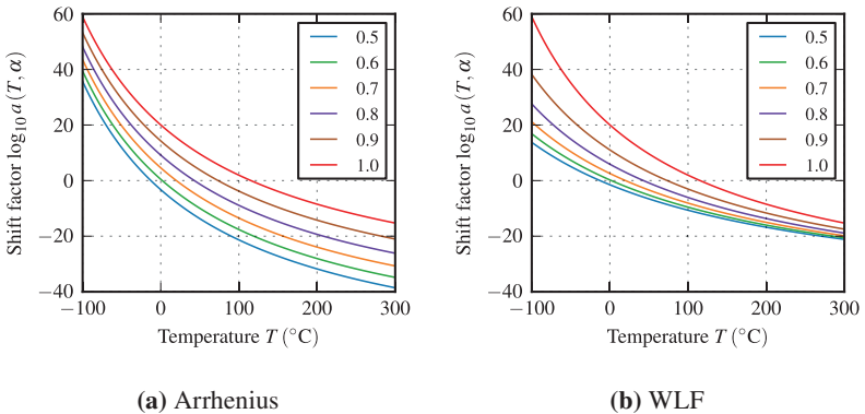
Figure 6.2: Comparison of Arrhenius and WLF based shift function formulations and different cure degrees. In both models, T_g(\alpha) is used as the reference temperature T_{ref} .
