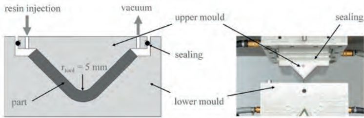
Figure 7.6: Visualization of the RTM setup used to manufacture L-shaped specimens (taken from Groh et al. [138])
