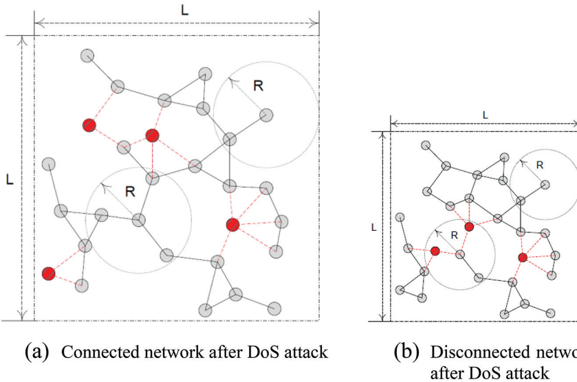
Figure 7.2 A connected ad hoc network with users independently and uniformly distributed in an L \times L grid. All users have “hearing distance” R , within which they can communicate with each other. Each user could potentially be affected by DoS. The users succumb to the attack are marked red and have to be removed, along with all associated links. The removal of the DoS victims could lead to either a connected or disconnected network.
