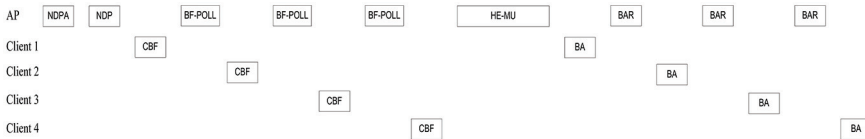
Figure 12.8 Downlink MU TXOP for 11ac.
