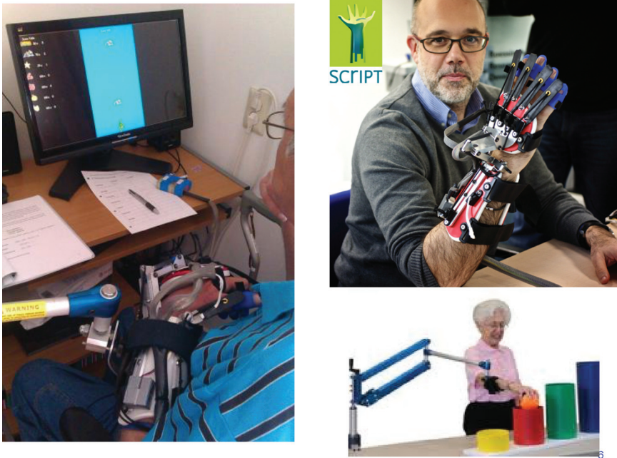
Figure 13.2 Upper extremity exercise system including robotic support for the hand functioning, gravity compensation and individually tailored video games (Scriptproject.eu).
