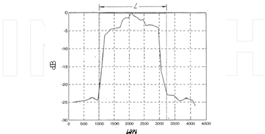
Fig. 14. Cross-talk measured on a single element at laser beam modulation frequency of 185 Hz.
