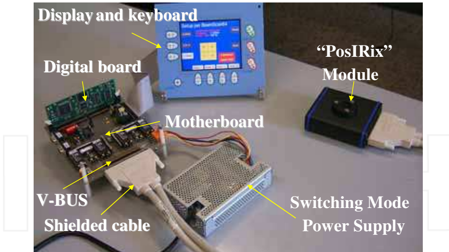
Fig. 21. Photograph of the components of the electronic instrument for IR laser beam characterisation
