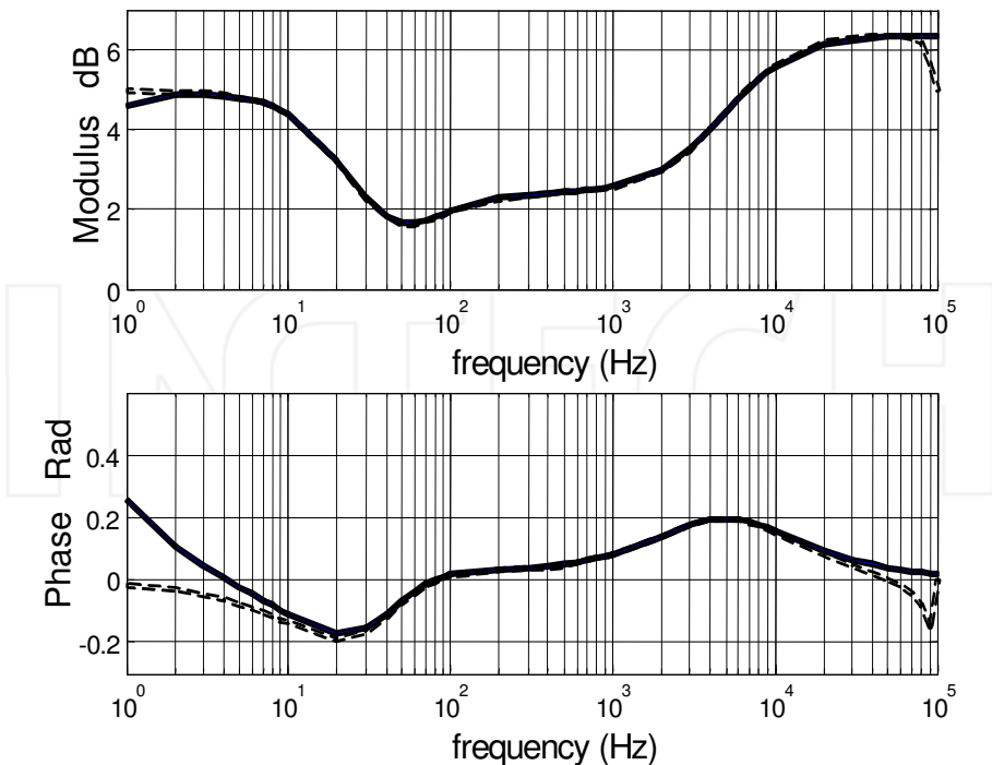
Fig. 28. Computed H_{\text{filt}} (continuous line) and numerical H_d (dashed line) implementations.
