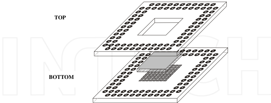
Fig. 12. Assembly for the pyroelectric matrix array.
