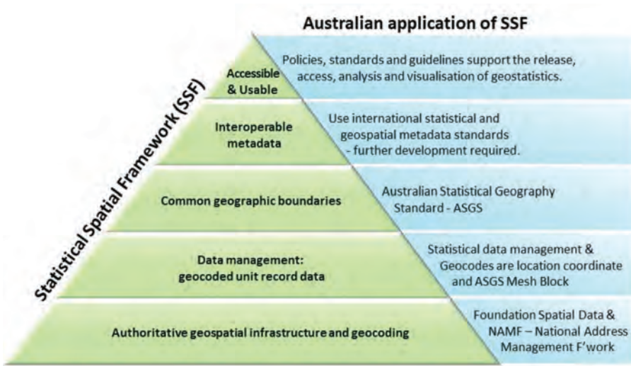
FIGURE 14.2 Australian Bureau of Statistics Statistical Spatial Framework
