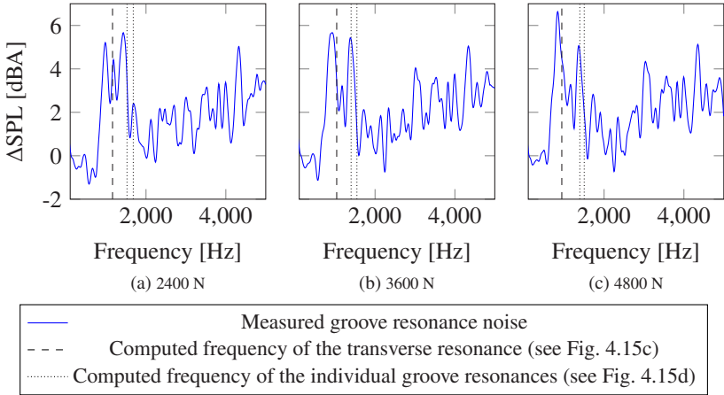
Figure 4.17: Comparison between measured and computed groove resonance frequencies of the winter tire (from [112])
