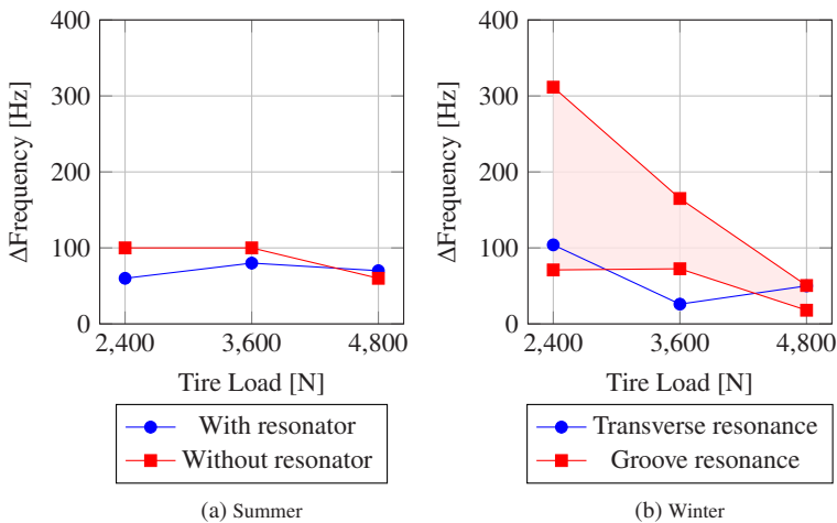
Figure 4.19: Drum curvature influence on the frequency shift of the computed groove resonance frequencies of the summer and the winter tires. The corresponding vibration shapes can be seen in Fig. 4.15.
