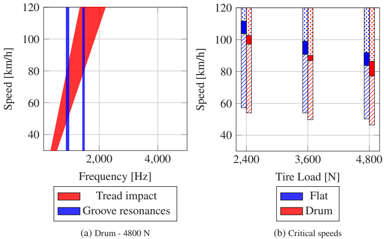
Figure 4.20: Drum curvature influence on the critical speeds for the summer tire. The dashed area corresponds to an interaction between the fundamental groove resonance and the tread pattern noise. The dotted area corresponds to an interaction between the second harmonic of the groove resonance and tread pattern noise. The filled area corresponds to an interaction between both groove resonance harmonics and tread pattern noise.
