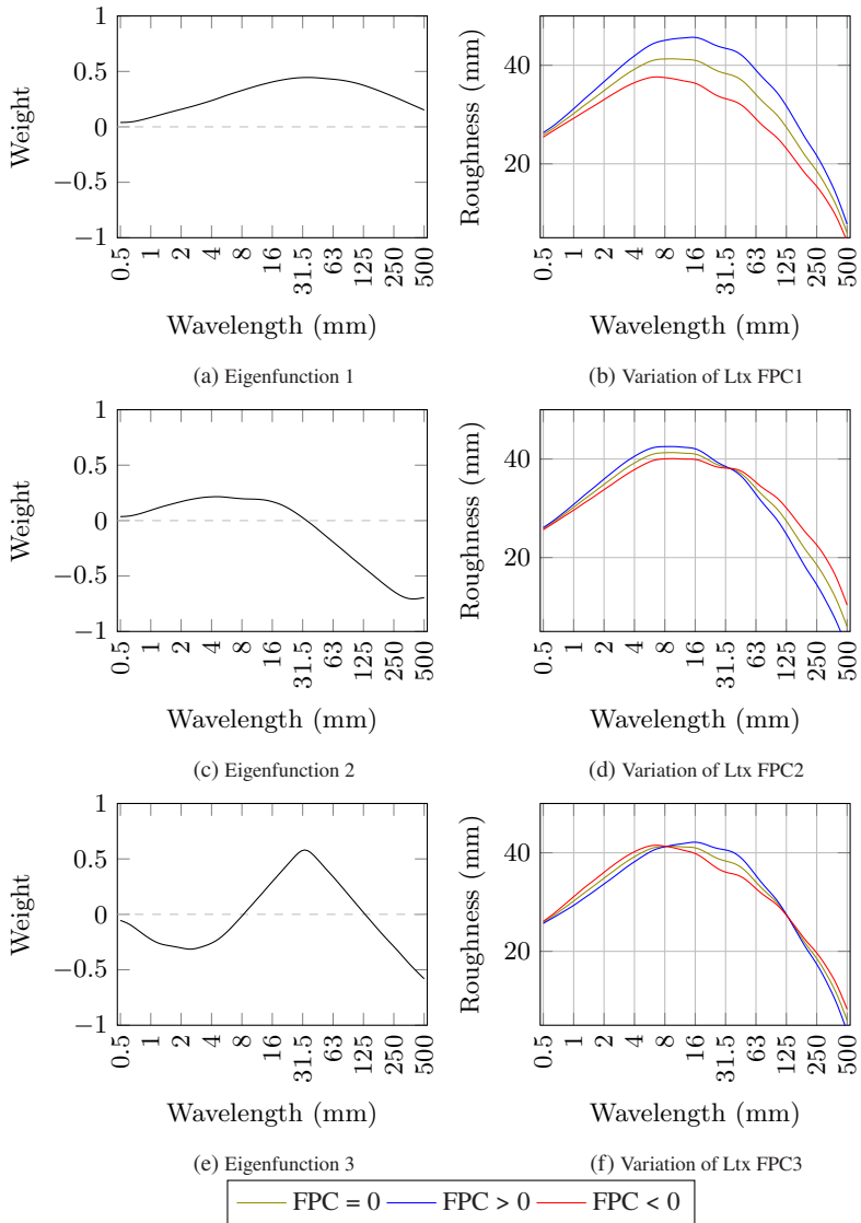
Figure 4.1: PPCA results for the texture amplitude spectrum for the field measurements. The left diagrams depict the eigenfunction of the roughness spectrum and the right diagrams show the influence of the FPC's sign on the spectrum.
