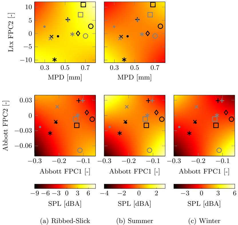
Figure 4.24: Influence of the significant road surface parameters interactions on TiRN on ISO 10844 test tracks using all parameters from the global road surface descriptors set. The relationship between the symbols and the test track number is given in Table A.6
