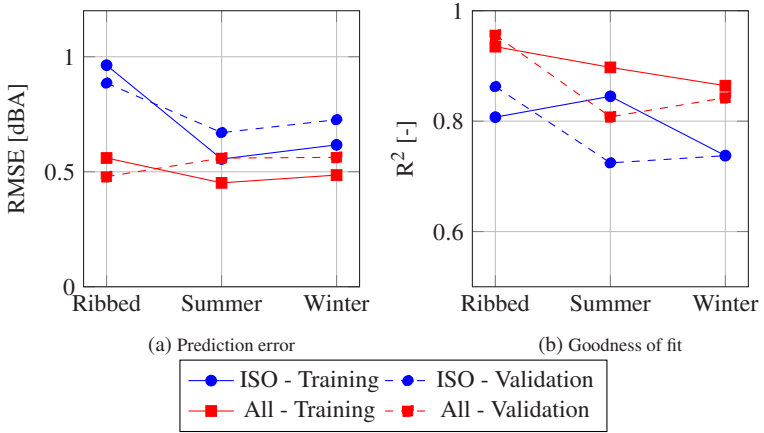
Figure 4.22: Comparison of the parameters data set on the goodness of fit and the prediction error on ISO 10844 test tracks. The drawn lines have no mathematical meaning and are used as guide to the eye
