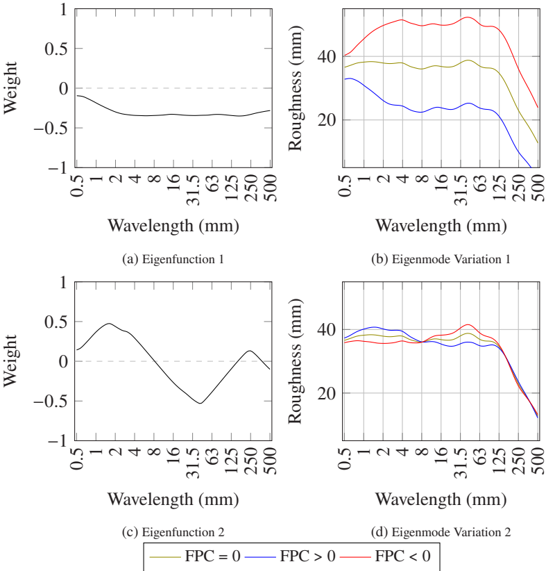
Figure A.2: Eigenfunctions of the principal components for the third-octave band spectra of the road surface roughness
