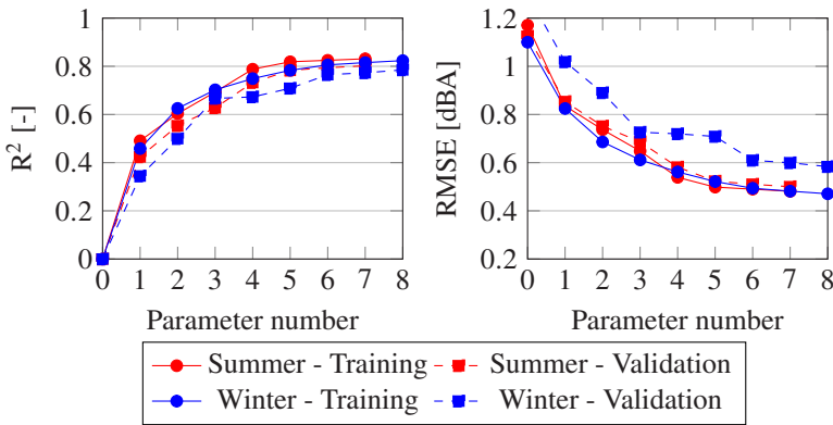
Figure 4.10: Influence of the number of parameters on the multiple linear regression goodness of fit and prediction error. The parameter number corresponds to the first column of Tables 4.2 and 4.1.
