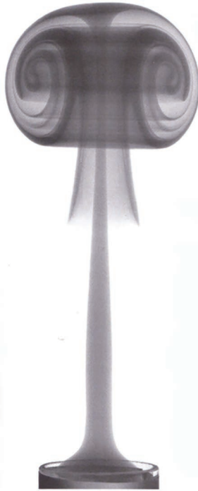
FIGURE 25.5 Ring vortex viewed from the side, made using marker dye in water, pushed in a slow pulse from the tube below. (Photo credit: by kind permission Andreas Wilkens, Institute of Flow Sciences, Herrschried, Germany, www.stroemungsinstitut.de .)
