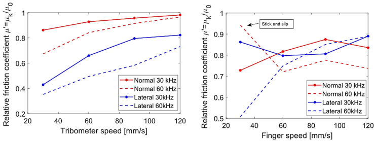
Fig. 4. Tribology measurements at 30 kHz vs. 60 kHz, at a vibration amplitude of 1.2 \mu\text{m}_{\text{p-p}} , and a pressing force of 0.5 N. Left: Tribometer measurements. Right: mean value of the measurements on a moving finger. Stick and slip was felt by the finger for normal vibration with a speed of 30 mm/s, which may explain the relatively high measurement. Moreover, active exploration with a moving finger may produce inaccuracies in the friction measurement of up to \pm 0.2
