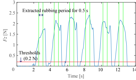
Fig. 3. Example of contact force for one trial. Two samples were rubbed alternatively for a total of 3 stroke for each. The data for the analysis was extracted for each stroke by using a threshold.
