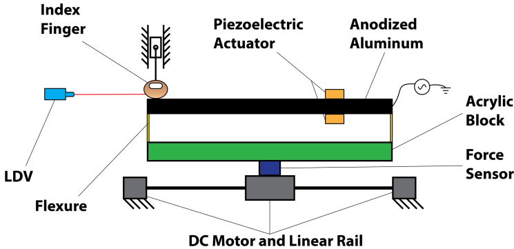
Fig. 2. Experiment platform.
