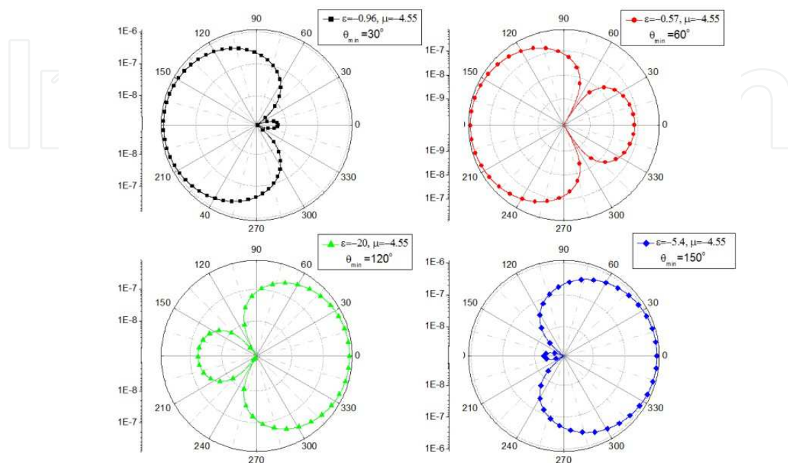
Fig. 7. Scattering diagrams of a spherical particle with a = 0.01\lambda and relative optical constants in the negative-negative range (labeled in the figure) which produce a minimum scattering at certain scattering angles. The particle is illuminated with a linearly polarized incident plane wave with the electric field perpendicular to the scattering plane (TE polarization).
