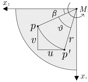
Figure 8.10: Rotation of a point p lying on a generic cross-section of the circular beam.
