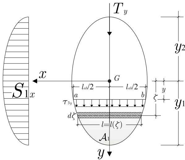
Figure 8.16: Symmetrical cross-section.
