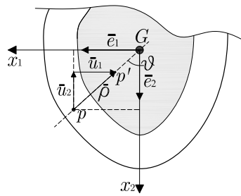
Figure 8.5: Strained state of a beam subjected to an axial force: radial contraction.
