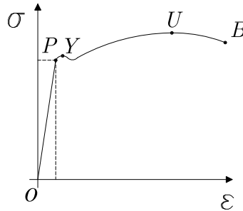
Figure 4.1: Hooke's law.
