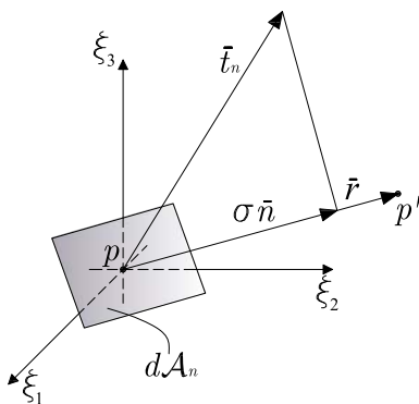
Figure 3.13: Stress quadratic of Cauchy.
