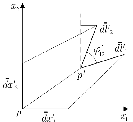
Figure 2.3: Angular dilatation.
