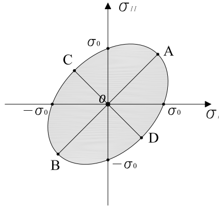
Figure 7.3: Elastic domain for Beltrami's criterion.
