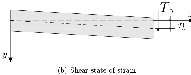
Figure 8.21: Two contributions to the state of strain for a beam subjected to terminal forces.
