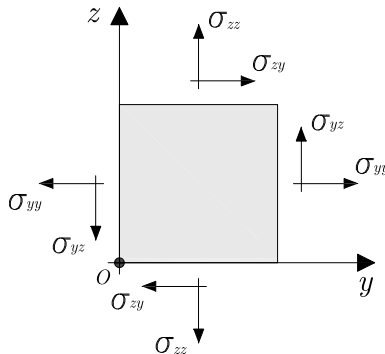
Figure 3.7: Plane (y, z) . Components of the stress tensor acting on the volume element.
