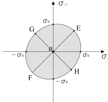
Figure 7.4: Elastic domain for the Mises' criterion.
