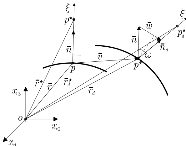
Figure 2.5: Two dimensional sketch of the displacement field for Kirchhoff–Love shells.
