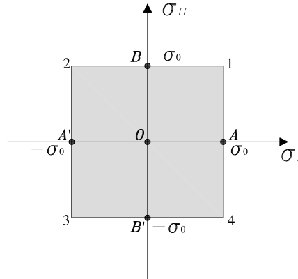
Figure 7.1: Rupture domain for the maximum stress criterion.
