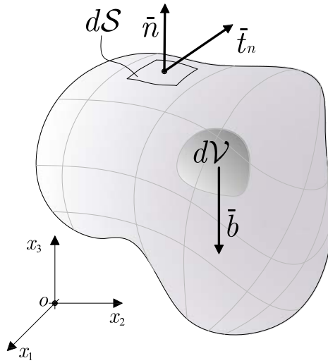
Figure 3.1: Body and surface forces.
