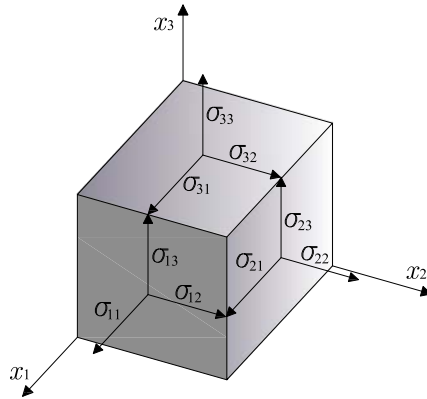
Figure 3.6: Stress tensor components acting on an infinitesimal volume element.
