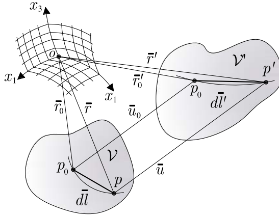
Figure 2.2: Measure of strain.
