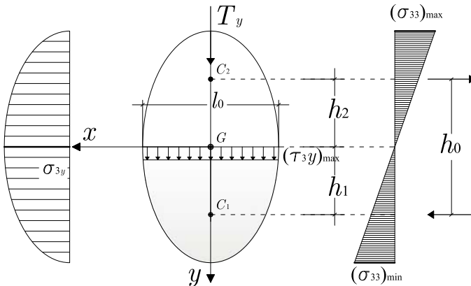
Figure 8.17: Maximum shear stress for symmetrical cross-section.
