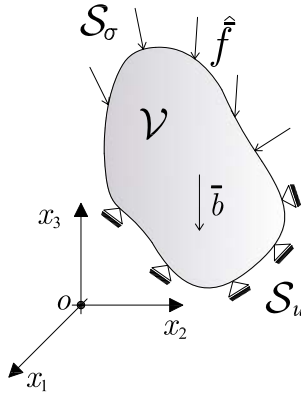
Figure 6.3: Forces and displacements acting on the body \mathcal{V} lying in the equilibrium state.
