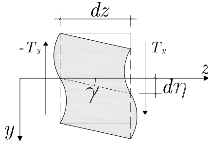
Figure 8.20: Shear strain for an infinitesimal beam segment.
