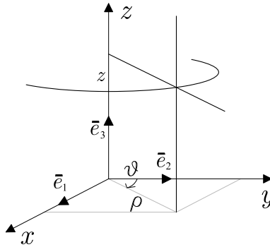
Figure 1.2: Cylindrical coordinate system.
