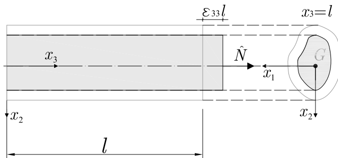
Figure 8.4: Strained state of a beam subjected to an axial force.
