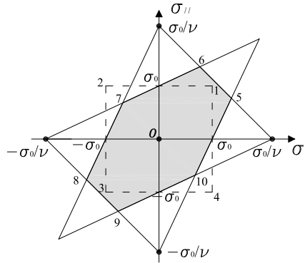
Figure 7.2: Rupture domain for the maximum strain criterion.
