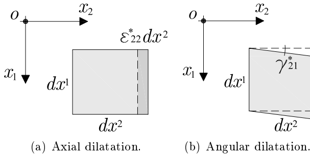
Figure 5.3: Virtual deformation.
