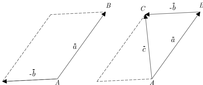
Figure 1.5: Subtraction of two applied vectors.
