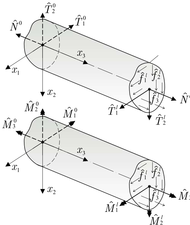
Figure 8.3: Equilibrated components of force and couple resultants acting on the ends of the beam.
