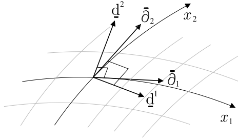
Figure 1.1: Contravariant and covariant bases related to a 2D curvilinear coordinate system.
