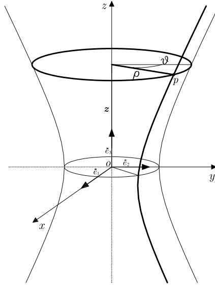
Figure A.1: Hyperbolic coordinate system.
