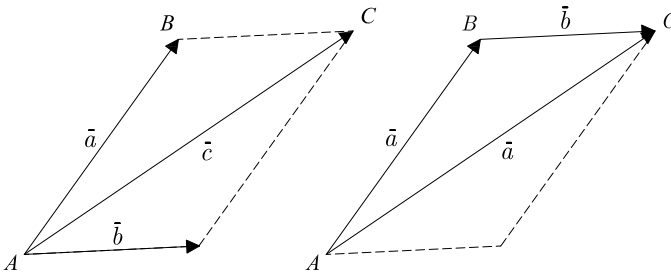
Figure 1.4: Addition of two applied vectors.
