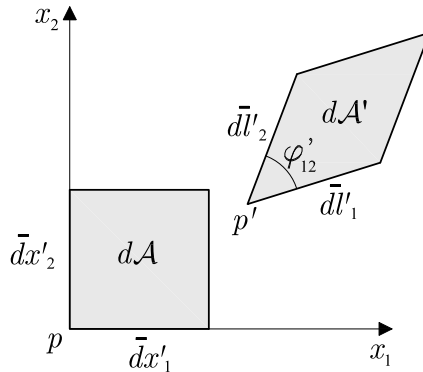
Figure 2.4: Area dilatation.
