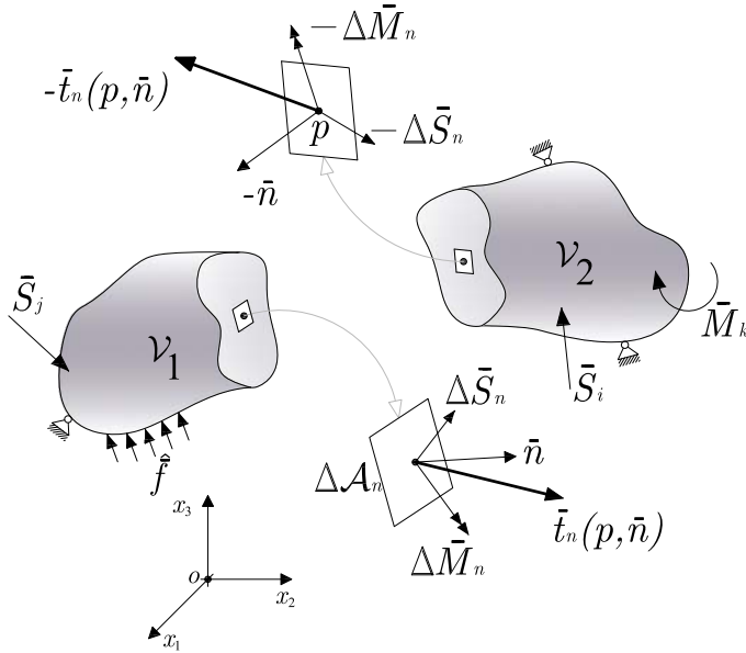
Figure 3.3: Splitting of the continuous media \mathcal{V} .
