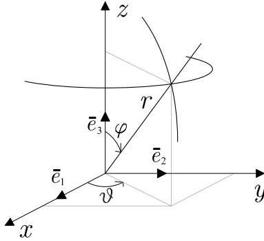
Figure 1.3: Spherical coordinate system.
