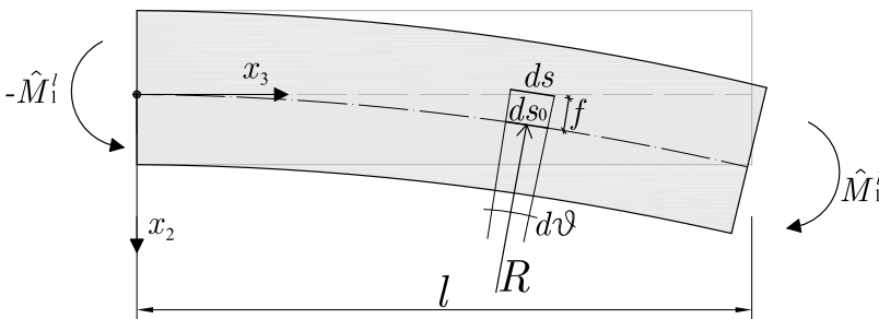
Figure 8.6: Beam under terminal couples.
