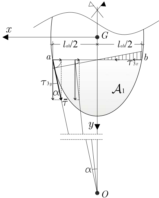
Figure 8.18: \sigma_{3x} distribution for symmetrical cross-sections.
