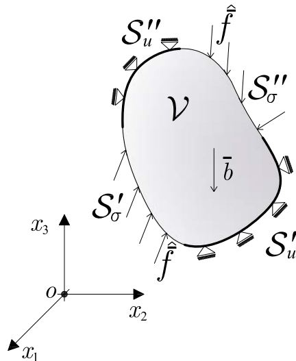
Figure 5.1: Forces and constraints acting on the continuum.
