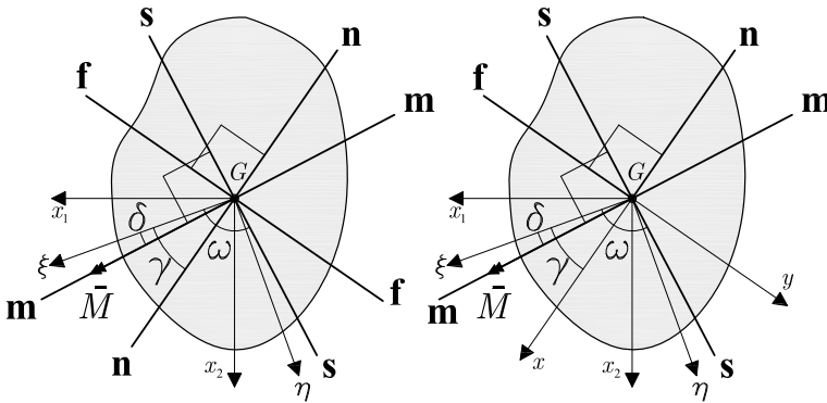
Figure 8.8: Neutral axis and flexural axis.
