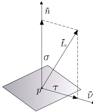
Figure 3.8: Normal and tangential components of the stress vector.
