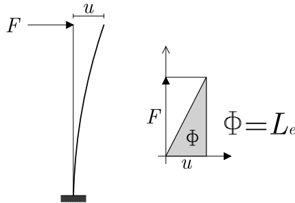
Figure 6.2: The simplest application of Clapeyron's theorem.
