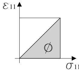
Figure 6.1: Density of strain energy in the case of axial state of stress.
