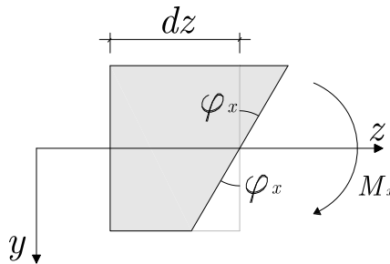
Figure 8.19: Bending strain for an infinitesimal beam segment.
