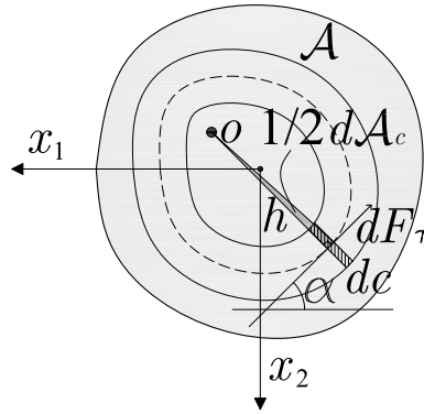
Figure 8.13: Stress resultants.
