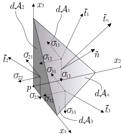
Figure 3.5: Stress tensor components.
