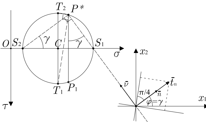
Figure 3.11: Graphical determination of principal directions.
