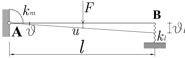
Figure 6.5: Example of Castigliano's theorems.
