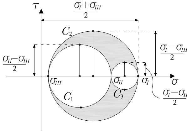
Figure 3.12: Mohr's circles.
