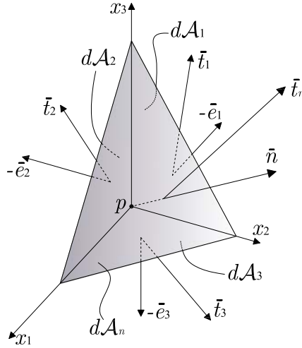
Figure 3.4: Stress vectors: the sketch of Cauchy's theorem.
