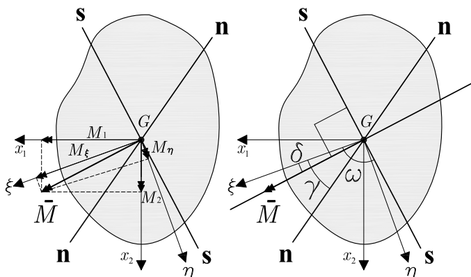
Figure 8.7: Projection of the couples and rotation axis.
