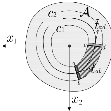
Figure 8.12: Stress flux within a small region included by two closed curves and two generic transversal sections.
