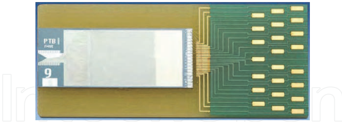
Fig. 5. Photo of a 10 V programmable Josephson junction series array.
