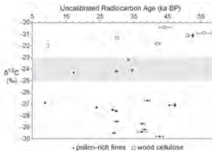
Figure 6. Radiocarbon age against \delta^{13}\text{C} (‰)
