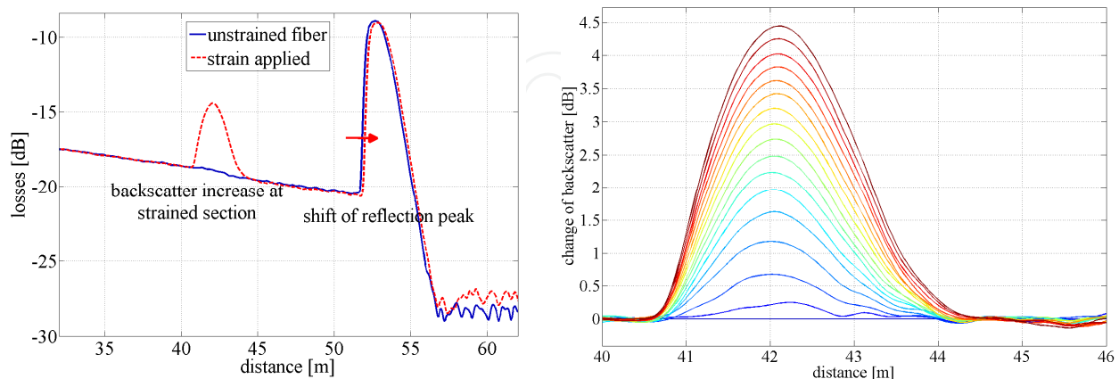
Figure 8. Left: OTDR trace of POF in unstretched condition (solid line) and of POF with a stretched fiber section at about 42 m (broken line). Right: Change of the scattering along a 1.4 m long POF section that is stretched from 0 to 16 % in steps of 1 %.
