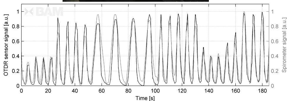
Figure 23. Monitoring of the respiratory abdominal movement of a human adult by POF OTDR sensor embedded in medical textiles (the OTDR sensor signal was compared with the signal measured by a spirometer).
