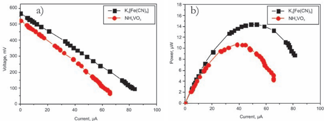
Fig. 2: a) Polarization characteristics and b) power curves obtained with 0.1 g/ml yeast + 250 mM glucose/67 mM phosphate buffer, pH 7 as an anolyte and 100 mM K_3[Fe(CN)_6] or NH_4VO_3 /67 mM phosphate buffer, pH 7 as a catholyte.
