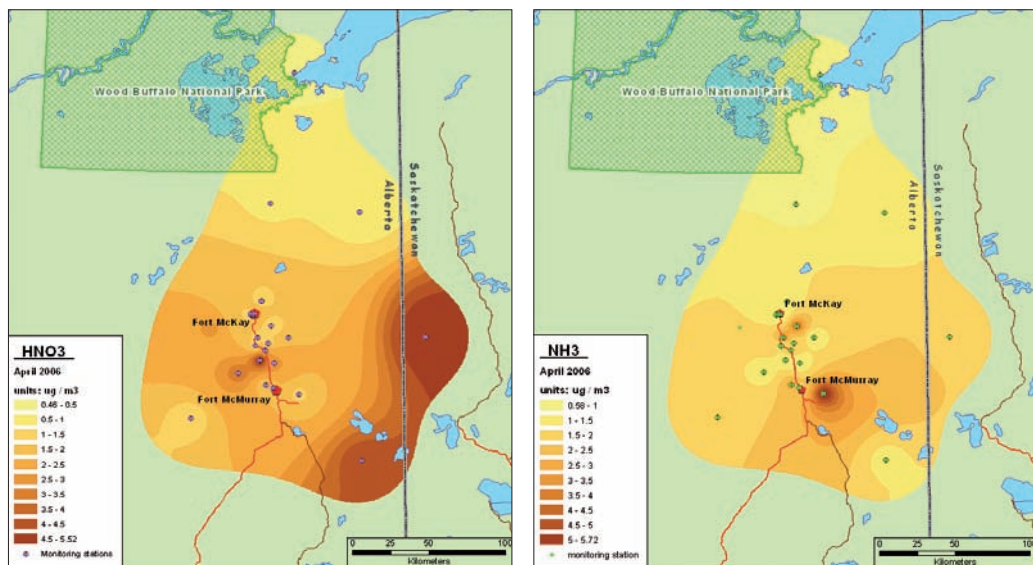
Fig. 6: Spatial distributions of \text{NH}_3 and \text{HNO}_3 are not correlated with each other for most of the monthly monitoring periods. This can be seen in the randomly selected example of April 2006.
