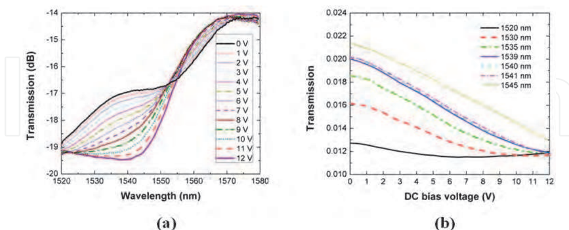
Fig. 13. DC characterisation results on a single pass (transmissive) EAM with an aperture of 100\ \mu\text{m} . The input optical power to the modulator is set at 0 dBm. (a) The transmission through the modulator (in decibels) as a function of the optical wavelength for different reverse bias voltages. (b) Transmission (in linear scale) as a function of the reverse bias voltage, for various optical wavelengths from 1520 nm to 1545 nm
