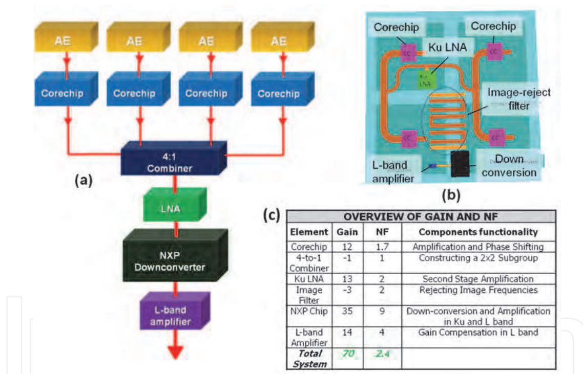
Fig. 11. (a) The configuration of the front-end. The corechip consists of an LNA and a 4-bit phase shifter. The NXP chip is used for downconversion and amplification. (b) Schematic layout of the RF front-end. (c) Overview of the gain and noise figure of the elements of the front-end chain.
