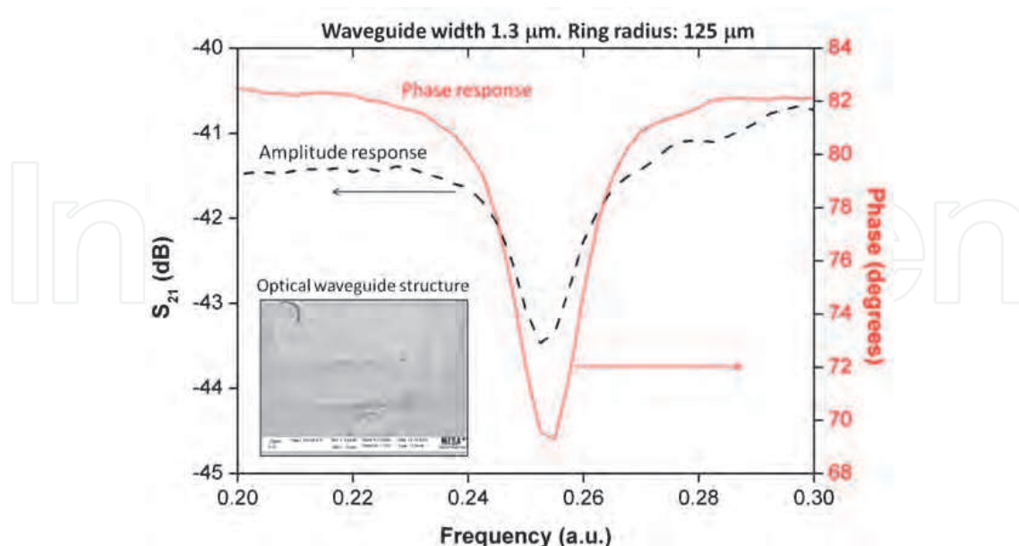
Fig. 15. Result of the propagation loss characterization of an optical ring resonator using the phase shift method. A loss of 0.2 dB/cm has been achieved. Inset: A scanning electron microscope (SEM) image of the waveguide cross-section.
