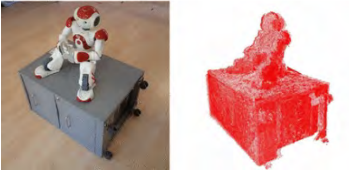
Figure 2.10: Reconstruction of a NAO robot by a NBV approach which considers sensor inaccuracies. Left: the real object. Right: the reconstructed point cloud. Figure taken from Vasquez-Gomez et al. (2017) (© 2017 Springer).
