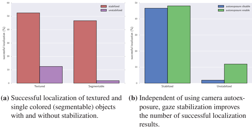
Figure 5.9: Number of successful object localization results. The experiment setup is illustrated in Figure 5.7. Left figure taken from Grotz et al. (2017a) (© 2017a IEEE).
