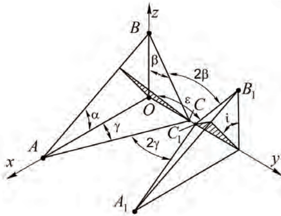
Figure 2.4. Schematic model of share lifter.
