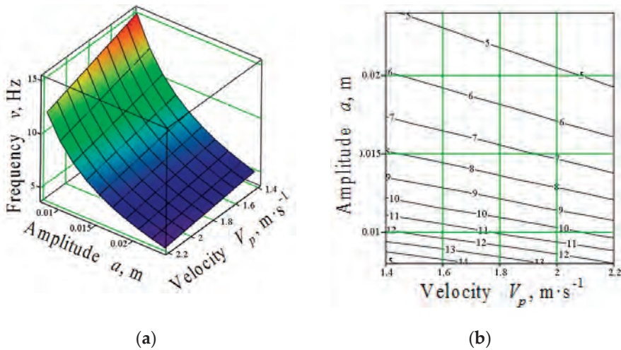
Figure 6.6. Surface (a) and contour diagrams (b) of values of digging tool oscillation frequency v = v(V_p, a) (Hz) that are acceptable under condition of not damaging roots in the case of their impact interaction with digging tool at two points.
