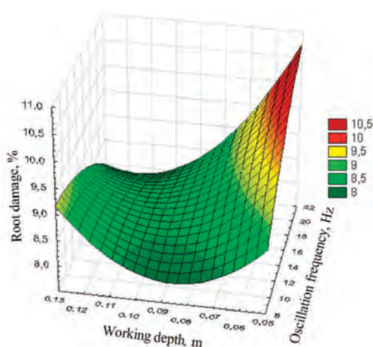
Figure 7.14. Quadratic response surface of root damage rate response to digging tool oscillation frequency and depth of its running in soil (at lifter translational motion velocity of 1.3 \text{ m}\cdot\text{s}^{-1} , soil hardness of 4.0 MPa, moisture content of 8.0%).
