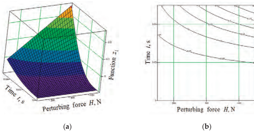
Figure 5.15. Surface (a) and profile graphs (b) of function z_1 = z_1(H, t) for the perturbing force amplitude's variation within a range of H = 100\text{--}700 N ( P_1 = 400 N, \nu = 10 Hz).
