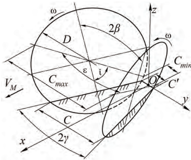
Figure 2.5. Schematic model of wheel lifter.
