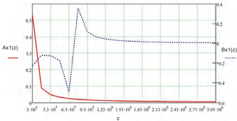
Figure 5.6. Graphs of relation between amplitudes of free A_{x,1} and free accompanying oscillations B_{x,1} along axis Ox_1 and soil's elastic deformation coefficient c ( H = 500 \text{ N} ; P_1 = 400 \text{ N} ; v = 10 \text{ Hz} ).
