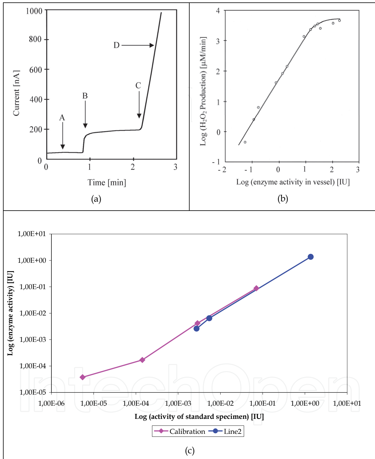
Fig. 12. a) Schematic view of enzyme activity measurement; A) addition of glucose concentration in vessel c_{\text{vessel}} = 500 \text{ mM} ; B) addition of H 2 O 2 for calibration c_{\text{vessel}} = 20.2 \text{ }\mu\text{M} ; C) injection of GOx solution of unknown activity; D) H 2 O 2 production (478 \mu\text{M}/\text{min} ). b) Calibration curve for enzyme activity measurement using MFS (Krejci et al., 2008). c) Calibration curve for enzyme activity measurement using RDE.
