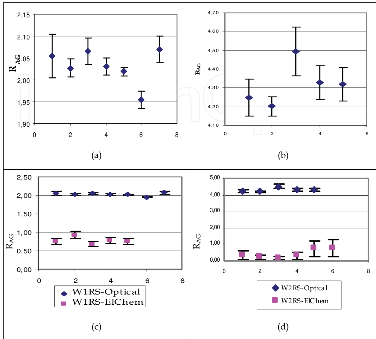
Fig. 3. The results of confocal microscope relation of active area to geometrical area ( R_{AG} ) measurement, a) ( R_{AG} ) for the sensor AC1.W1.RS (Au) b) ( R_{AG} ) for the sensor AC1.W2.RS (Pt). Comparison with electrochemical measurement c) Sensor AC1.W1.RS (Au) d) Sensor AC1.W2.RS (Pt).
