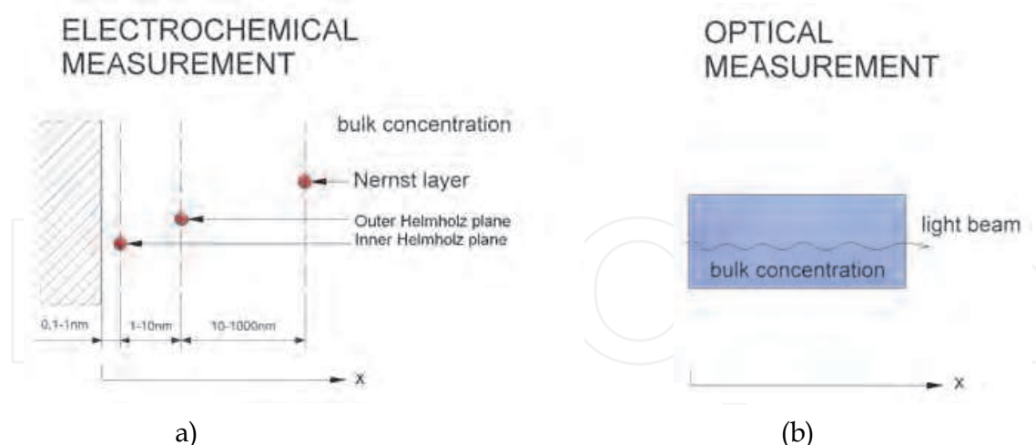
Fig. 1. Difference between electrochemical (a) and optical (b) measurement.
