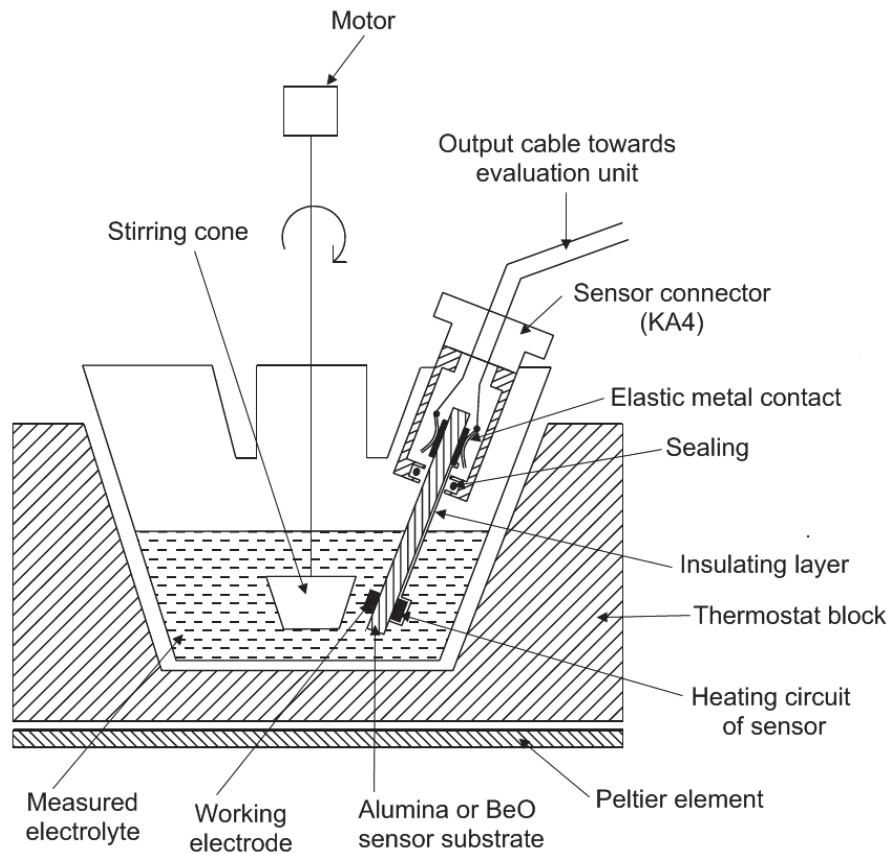
Fig. 8. Schematic of the Soret system (the gap between the cone and electrode surface is 1 mm)
