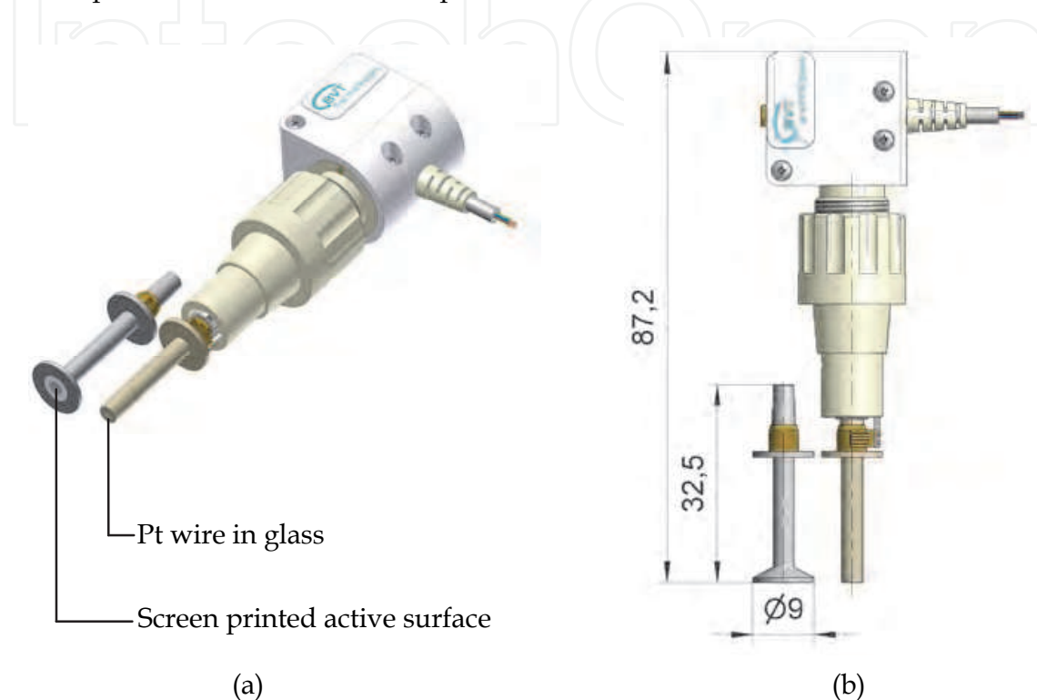
Fig. 7. a, b) Mini-rotated disc electrode
