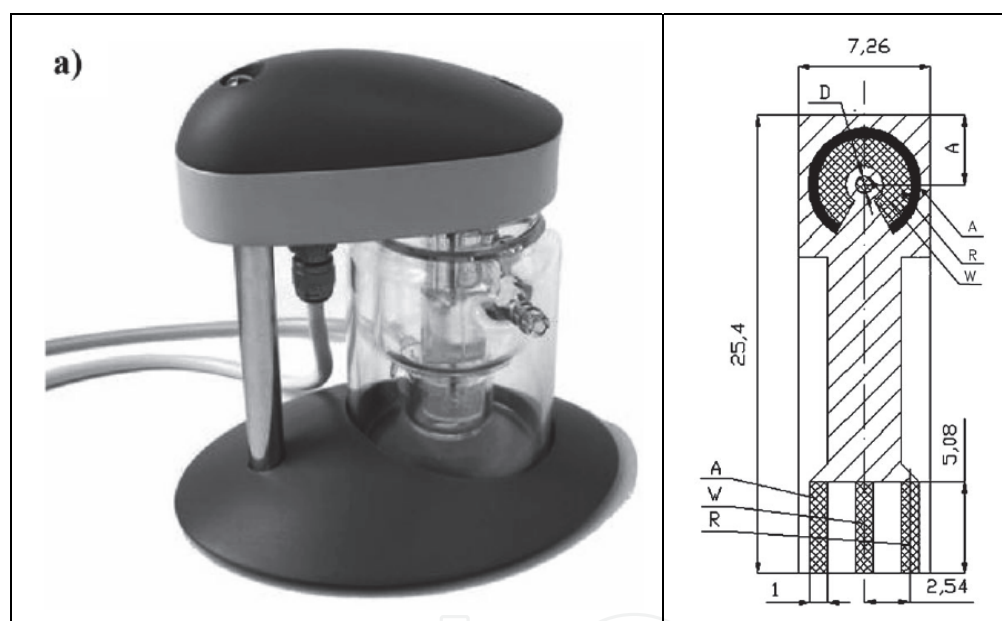
Fig. 6. a) Photo of the microflow system (MFS) device (BVT Technologies, a.s., Czech Republic). b) Integrated three-electrode amperometric sensor (Patent CZ 291411) (A: auxiliary electrode, R: reference electrode, W: working electrode) (Krejci et al., 2008).
