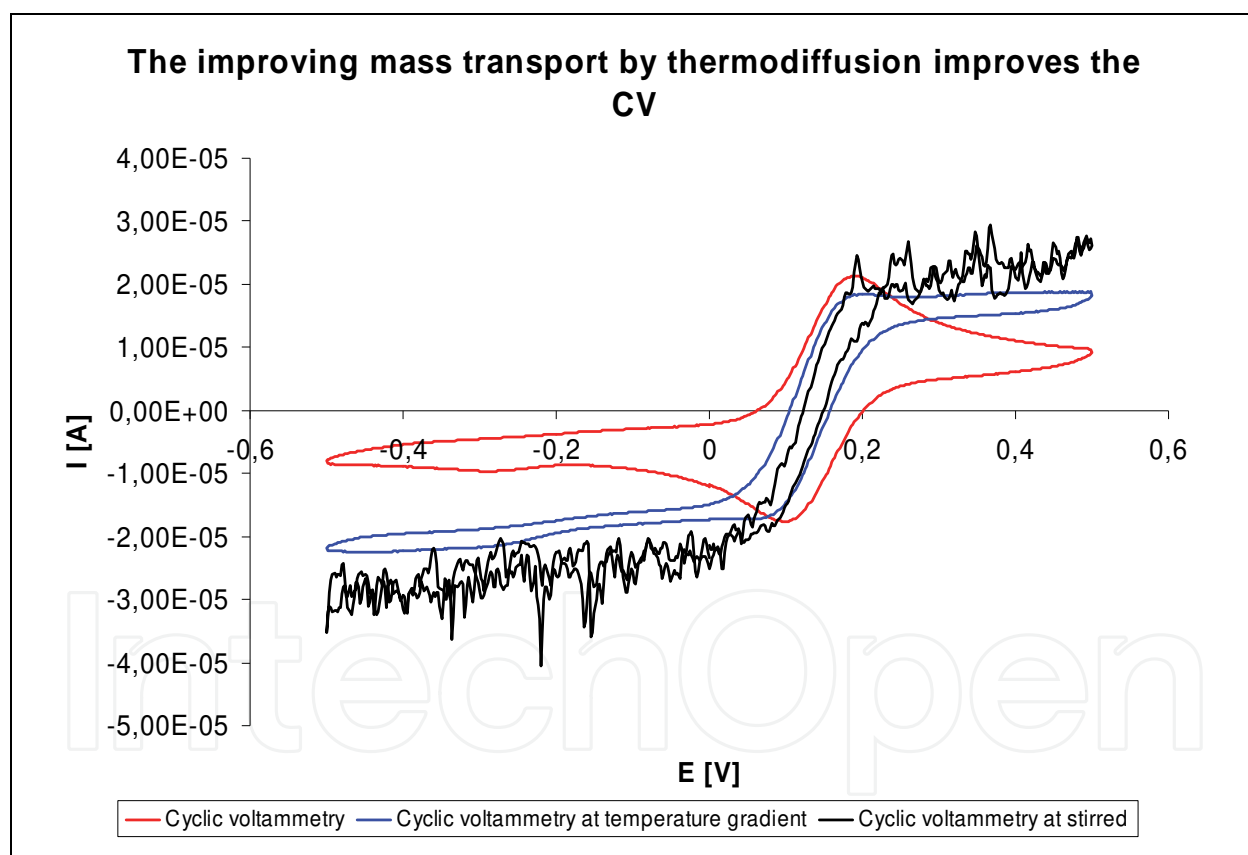
Fig. 13. The improving of mass transport by thermo diffusion
