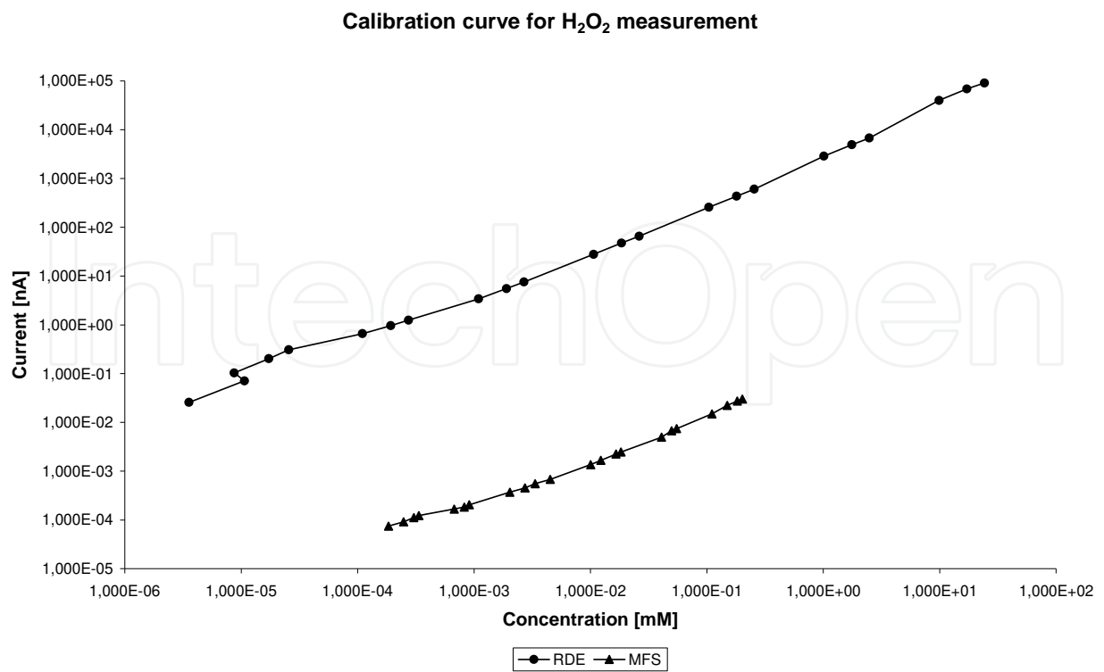
Fig. 9. Calibration curve for H 2 O 2 measurement (Krejci et al., 2008).
