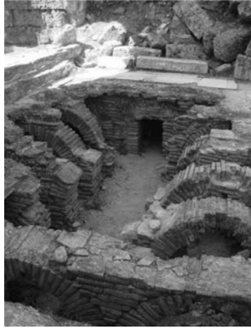
Figure 13.30 Hypocaust of the hot baths in Perge
