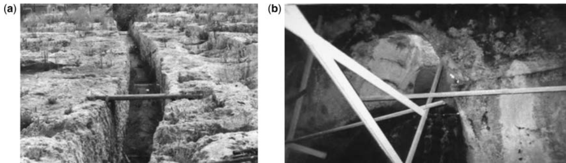
Figure 14.5 Water system at Syracuse: (a) view of aqueduct above grottoes and (b) outlets of the Galermi and Ninfeo aqueducts inside grotto formation (with permission of Mays et al. 2007)
