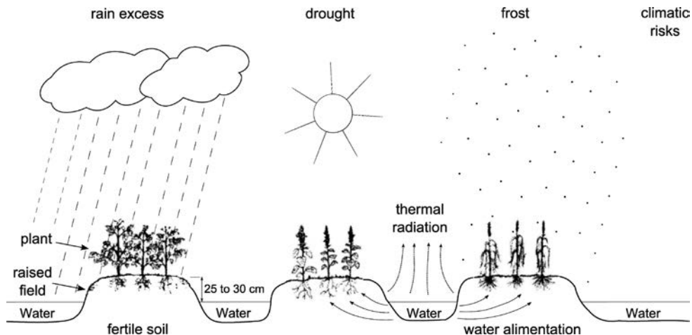
Figure 11.13 Raised-field (“waru waru”) farming technique utilised by the Tiahuanaco civilization, and still in use nowadays in the Peruvian and Bolivian Altiplano (Drawn after Canahua Murillo, 1992)
