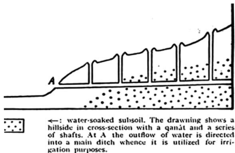
Figure 6.9 Qanat diagram
