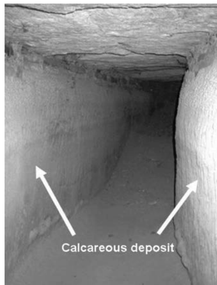
Figure 13.17 Picture taken from the inside of a masonry channel inside the city of Apamea. Calcareous deposits on the channel inner walls can be observed
