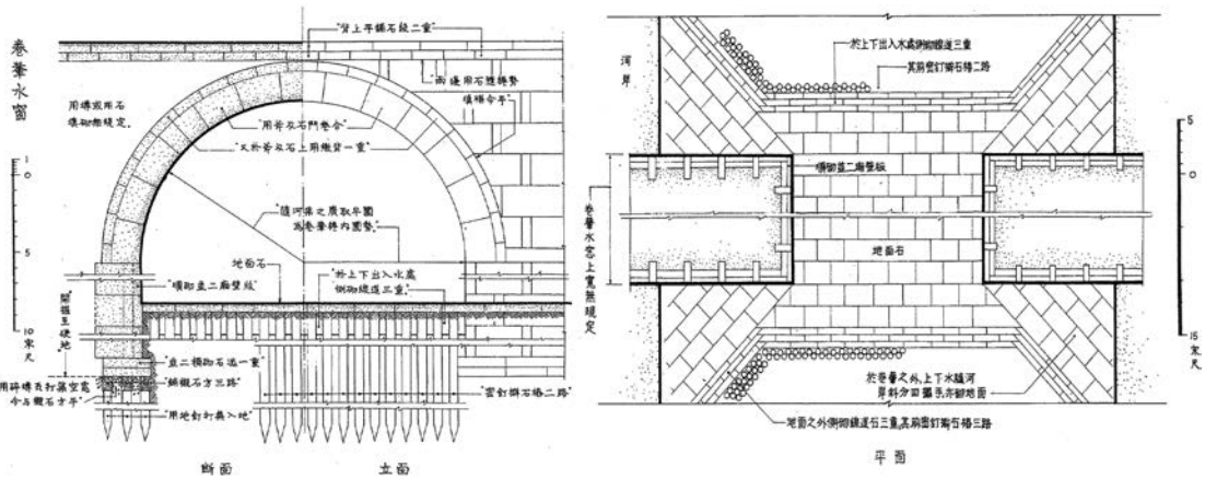
Figure 8.43 Cross and plan section of arched water gate according to “Yingzao fashi” by Li Jie, Song Dynasty, 1103 (Liang Sicheng, 1983)
