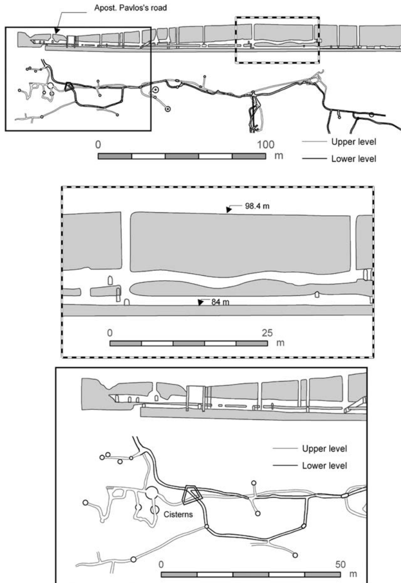
Figure 16.10 Top: general plan and section of the underground hydraulic works in Dörpfeld's excavation. The basin-like shape of the upper gallery is obvious in the middle; details of the complex of conical cisterns, wells and galleries is shown at the bottom (Gräber, 1905)
