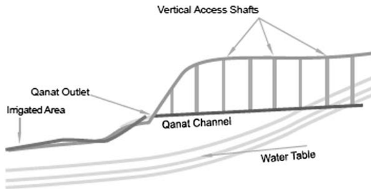
Figure 5.7 Qanat constructions
