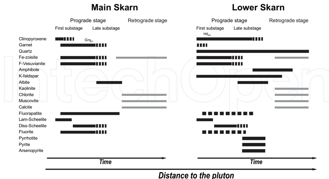
Figure 8. Paragenetic sequence of the Tabuaço scheelite skarn, showing the evolution of the mineral associations versus time and versus distance to the pluton (i.e. for the two skarn horizons).
