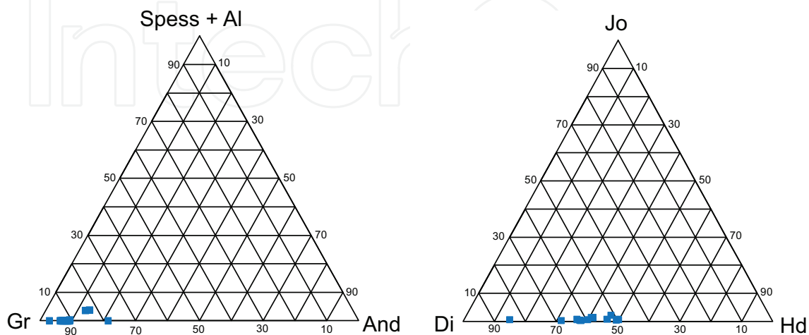
Figure 6. Ternary diagram showing composition of garnets from the Main Skarn, between andradite (And), grossular (Gr) and spessartine + almandine (Spess + Al) (left), and composition of clinopyroxene from the Lower Skarn, between hedenbergite (Hd), diopside (Di) and Johannsenite (Jo) (right).
