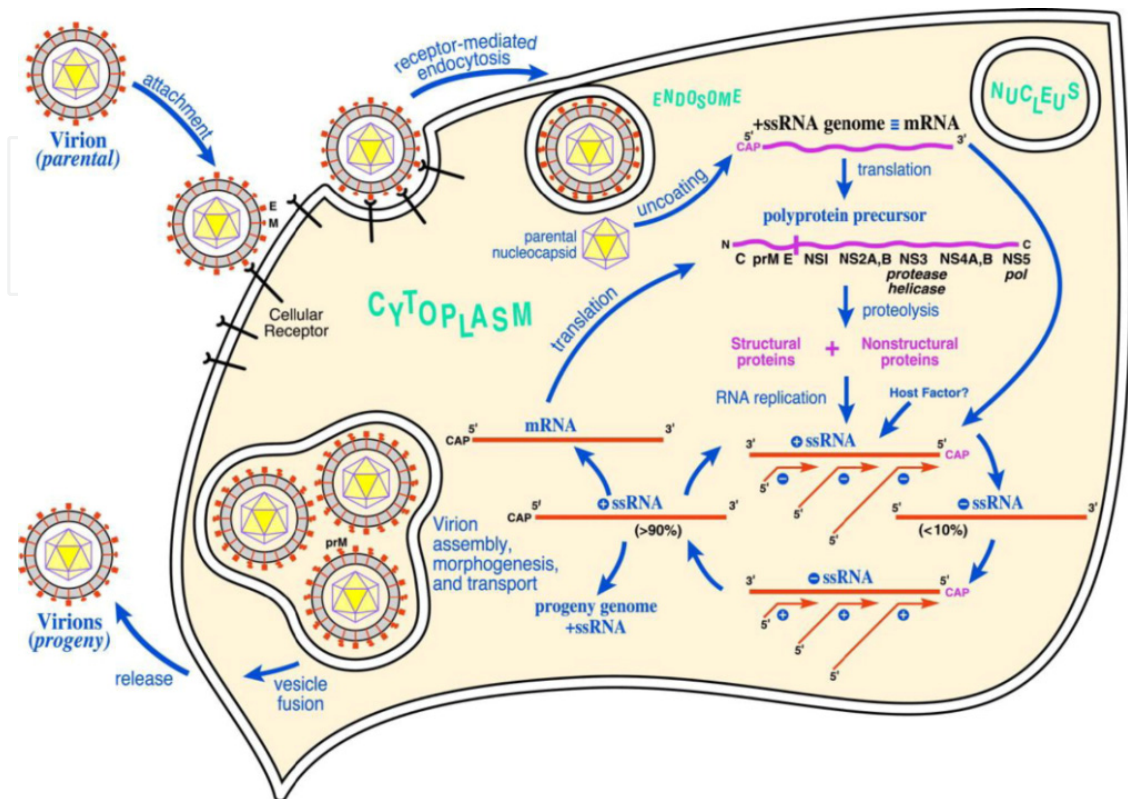
Figure 4. West Nile virus replication cycle. The virion is attached to the cellular receptors, and the envelope fuses with the membrane. The viral RNA is released by the nucleocapsid with a yet unknown mechanism and serves as mRNA for translation of all viral proteins and as template during RNA replication. Virion assembly and release of them to the extracellular milieu complete the replication cycle. Reprinted with permission from PNAS 2002, vol. 99 no. 18 11555-11557. Copyright 2002 National Academy of Sciences, U.S.A.
