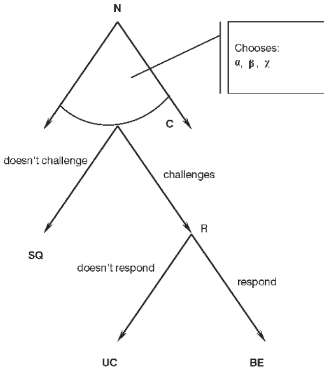
Figure 1.1 Basic structure of the game
